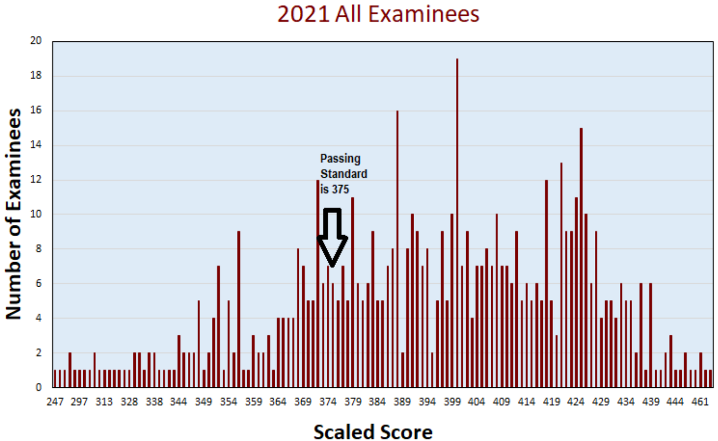
Graph 1. All 2021 Examinees
