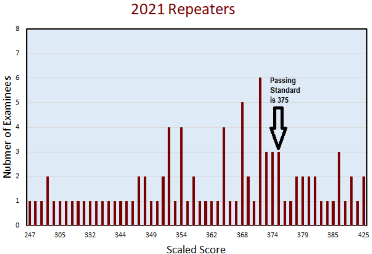
Graph 3. 2021 Repeat Examinees
